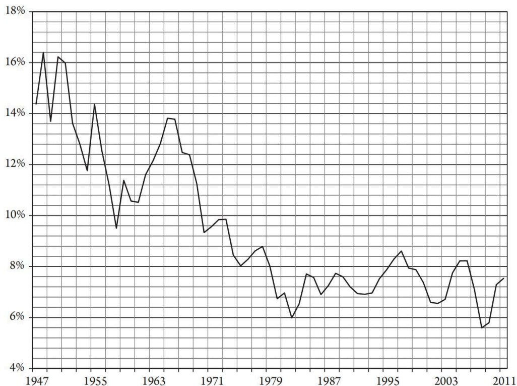
Figure 2.11 US Corporate Rate of Profit 1947–2011 知乎 @ 最遥远的路
